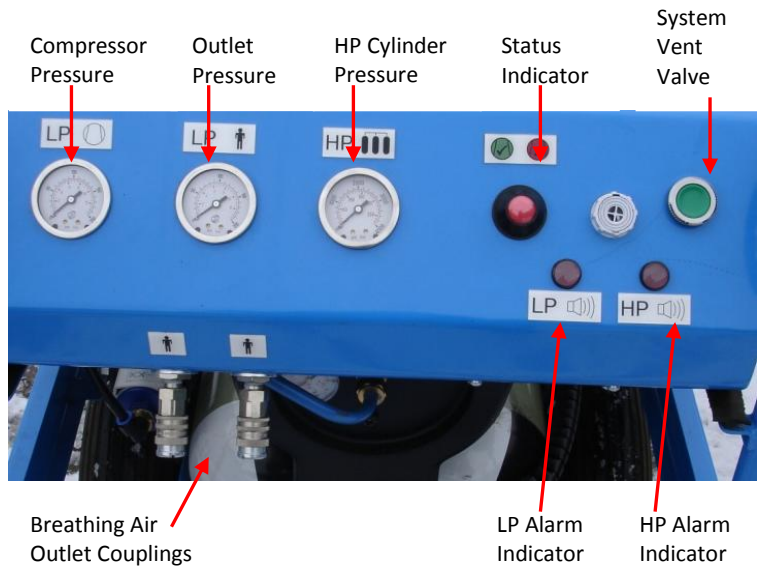
Below – BA20E Control Panel
